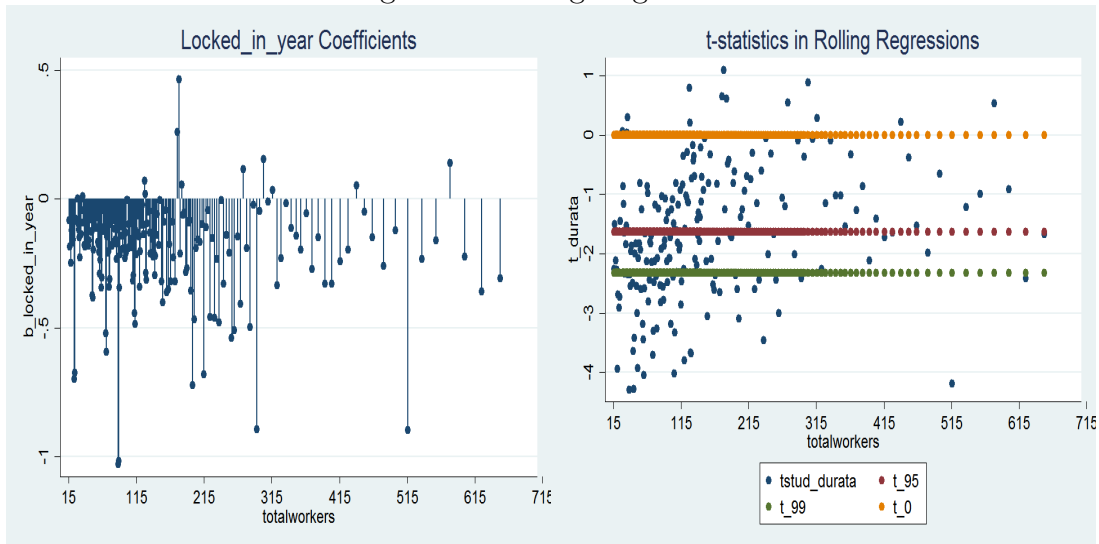
Figure 5: Rolling Regression
